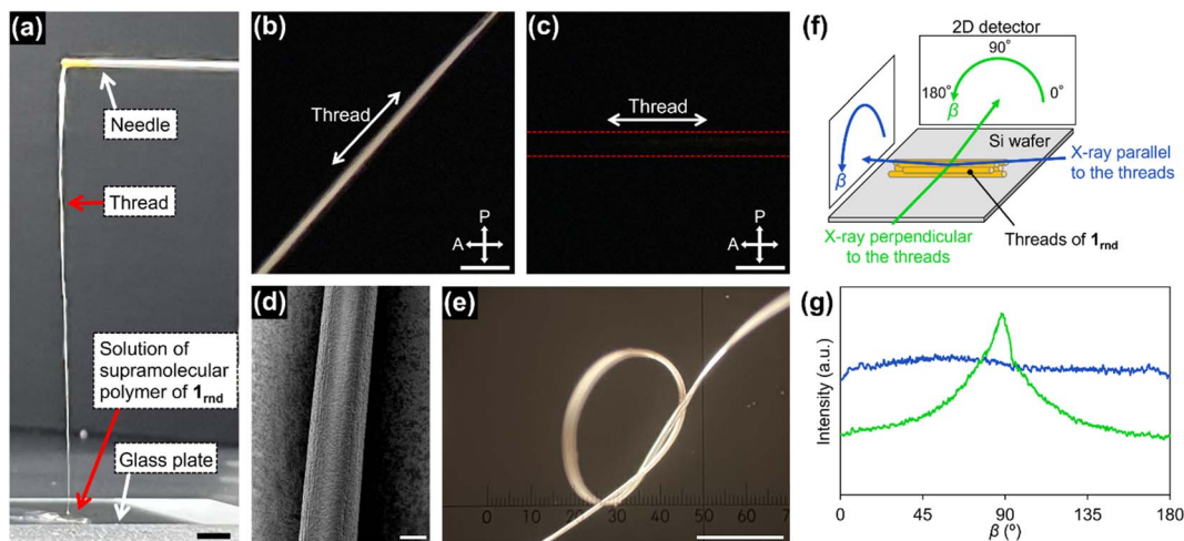
Fig. 5 (a) Photograph of a thread drawn from a concentrated solution of 1_{\text{rmd}} prepared by seeded polymerization (Fig. 3d): scale bar = 5 mm. POM images of the thread on a glass substrate with the thread rotated (b) 45^\circ and (c) 0^\circ/90^\circ with respect to the polarizer/analyser: scale bar = 100 \mu\text{m} . (d) SEM image of the thread: scale bar = 20 \mu\text{m} . (e) Optical micrograph of a knotted thread: scale bar = 500 \mu\text{m} . (f) Schematic representation of the experimental setup for 2D GI-WAXD. (g) Angle-dependence of the peak intensity for 2\theta = 1.7^\circ - 2.7^\circ (ca. 3.9 \text{ nm} ) in the 2D GI-WAXD with respect to \beta , as shown in (f).
