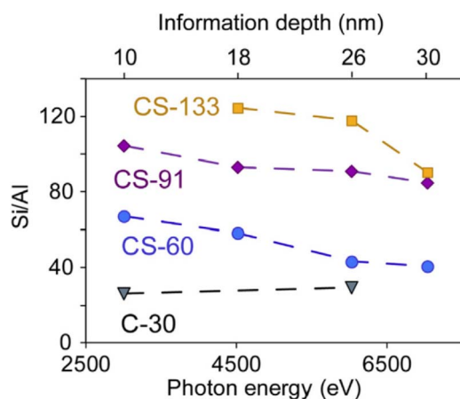
Fig. 6 Comparison of Si/Al ratios for a ZSM-11 core (C-30 with Si/Al = 30) and core-shell samples (CS-60, CS-91, and CS-133), and the corresponding Si/Al ratios of the shell are 60, 91, and 133 from XPS depth analysis (VKE-XPS) as a function of photon energy (bottom x-axis) and the corresponding information depth (top x-axis) where 95% of the signal is generated. Each sample was pre-coated with ca. 10 nm of carbon. Any uneven (or rough) surfaces of zeolite powders from VKE-XPS sample preparation increase the uncertainty in depth estimation for a single particle. This results in a diffuse transition between the shell and core that creates uncertainty in estimates of shell thickness. Reproduced from ref. 173 with permission from Elsevier, Copyright 2022.
