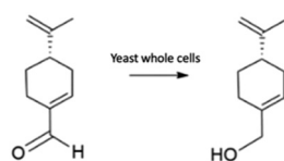
Scheme 1 Reduction of ( S )-perillaldehyde into ( S )-perillyl-alcohol.
