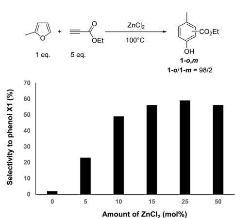
Fig. 4 Impact of the amount of \text{ZnCl}_2 on the selectivity to phenol 1 (at 95% conv. of MF) (MF (1 eq.), ethylpropiolate (5 eq.), 100 °C).
