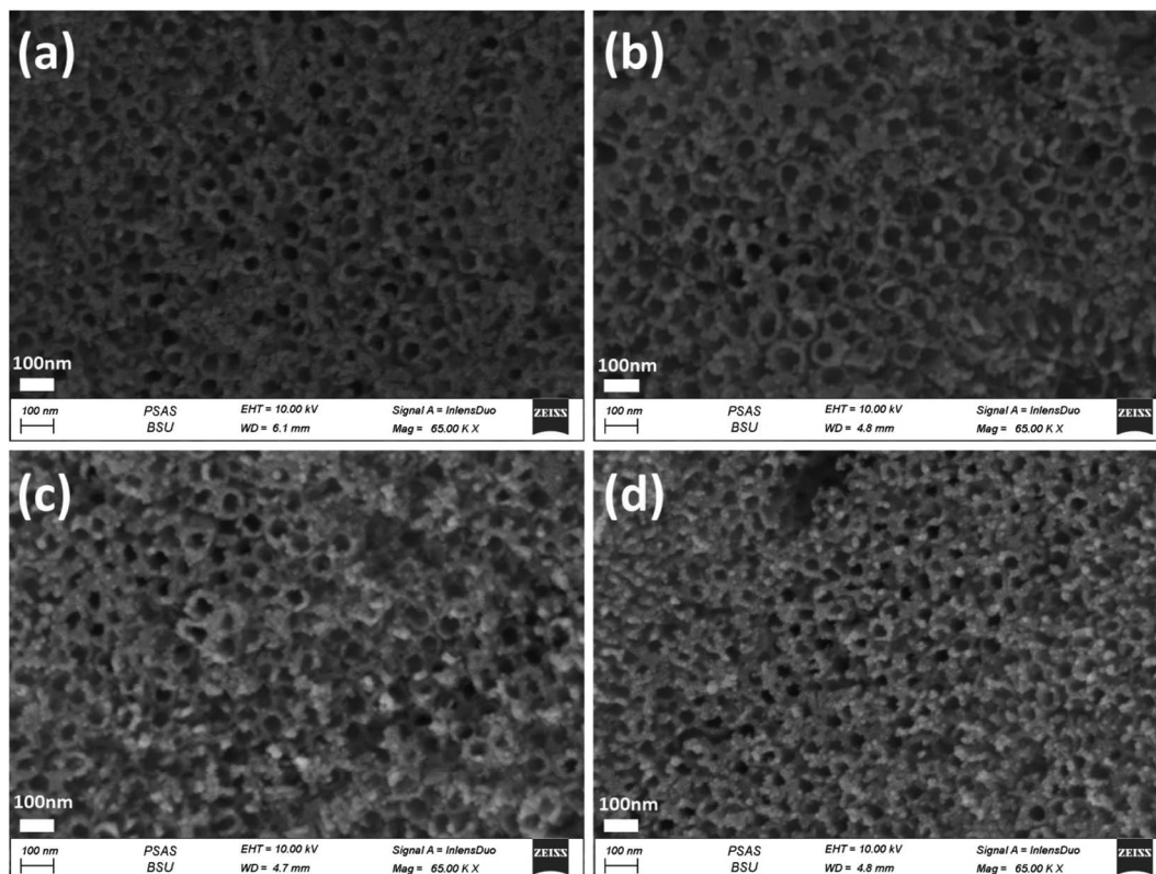
Fig. 4 FESEM images of the top-view of Au 30 /Ni 20 /TiO 2 NTs photoanodes synthesised by different time intervals of photodeposition (a) 15 min, (b) 30 min, (c) 60 min and (d) 120 min.
