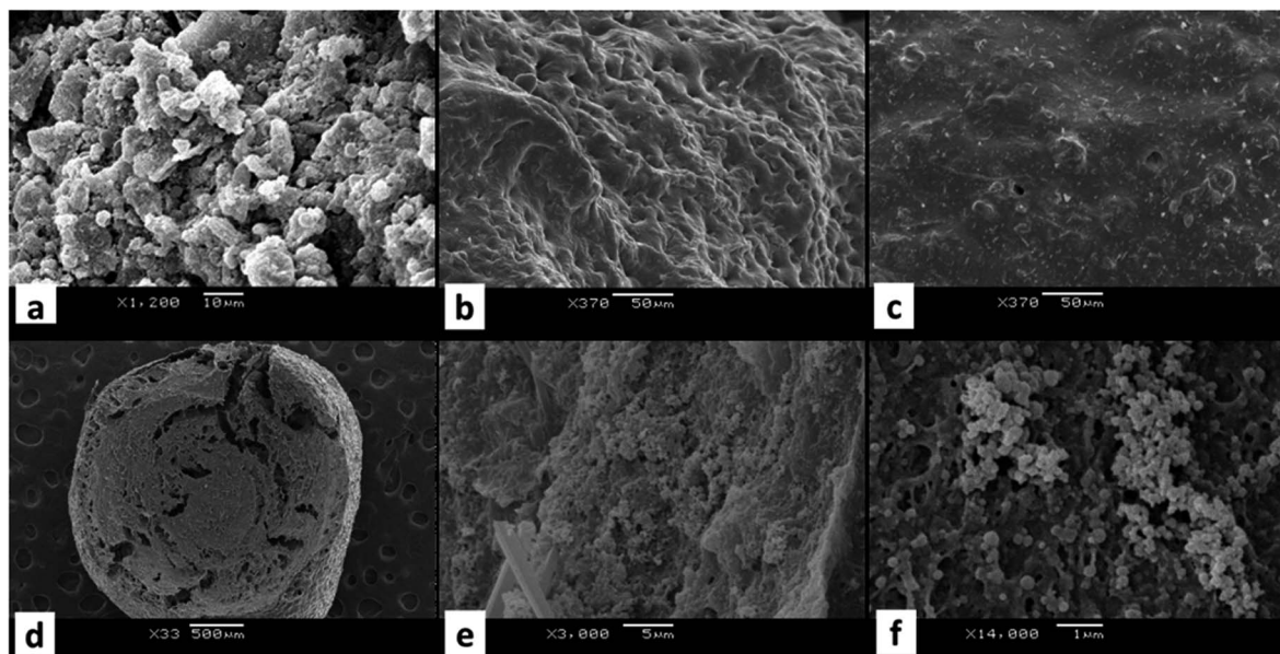
Fig. 3 Scanning electron micrograph of (a) starting biomaterial used to form the hydrogel beads from the treatment of switchgrass, (b) surface of freeze-dried hydrogel beads based on switchgrass biomaterial, (c) surface of hydrogel based on switchgrass with entrapped laccase, (d) a cross-section of the bead of hydrogel with entrapped laccase, (e and f) magnification of the cross section shown in (d).
