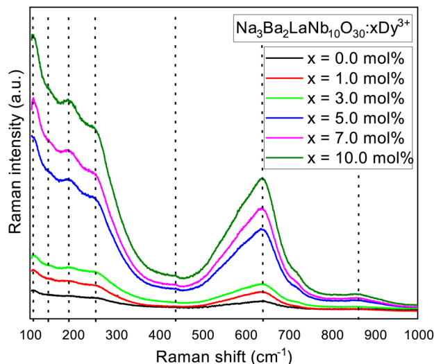
Fig. 7 Raman spectrum of \text{Na}_3\text{Ba}_2\text{LaNb}_{10}\text{O}_{30}:\text{x}\text{Dy}^{3+} ( x = 0, 1, 3, 5, 7 and 10 \text{ mol\%} ) phosphor at room temperature.
