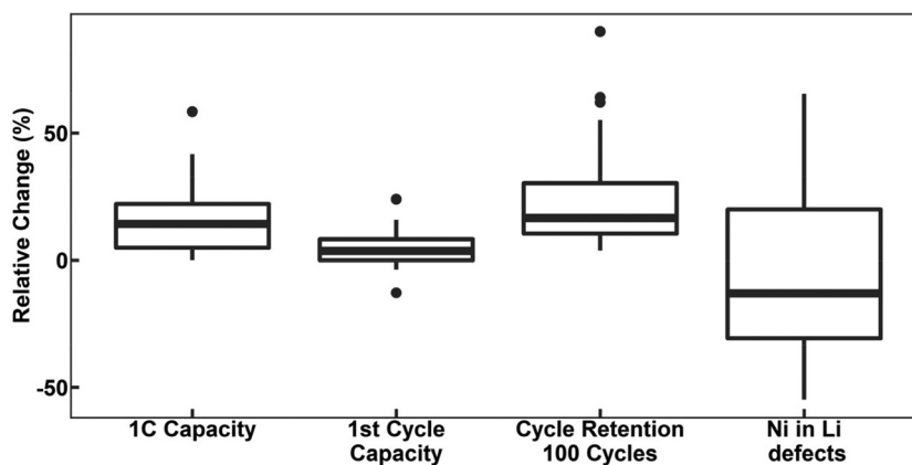
Fig. 7 Box-and-whisker plot of the relative change of 1C capacity ( n = 16 ), first-cycle capacity ( n = 22 ), capacity retention after 100 cycles ( n = 22 ), and \text{Ni}_{\text{Li}}^{\cdot} defects ( n = 11 ) of Nb-doped LTMOs applied for LIBs.
