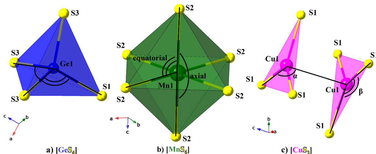
Fig. 5 (a) [\text{GeS}_4] tetrahedral unit showing \angle\text{S3-Ge-S1} and \angle\text{S3-Ge-S3} angles; (b) [\text{MnS}_6] octahedral unit showing \angle\text{S2-Mn-S2-axial} and \angle\text{S2-Mn1-S2-equatorial} angles; (c) two [\text{CuS}_3] trigonal planar units showing angle \alpha ( \angle\text{Cu1-Cu1-S2} ) indicating the co-planarity of these two units (perfect co-planarity having \alpha = 90^\circ ), and angle \beta ( \angle\text{S2-Cu1-S2} ) indicating the deviation from the planar D_{3h} ( \bar{6}m2 ) symmetry for [\text{CuS}_3] (in planar \beta = 120^\circ ).
