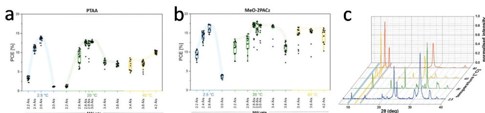
Fig. 7 Box plot of power conversion efficiency extracted from J – V scans (reverse and forward) measured under simulated AM 1.5G illumination for solar cells prepared at different substrate temperatures and MAI rates on (a) PTAA and (b) MeO-2PACz. (c) Normalized XRD patterns of co-evaporated films on PTAA deposited with different substrate temperatures. Reproduced with permission. 101 Copyright 2020, American Chemical Society.
