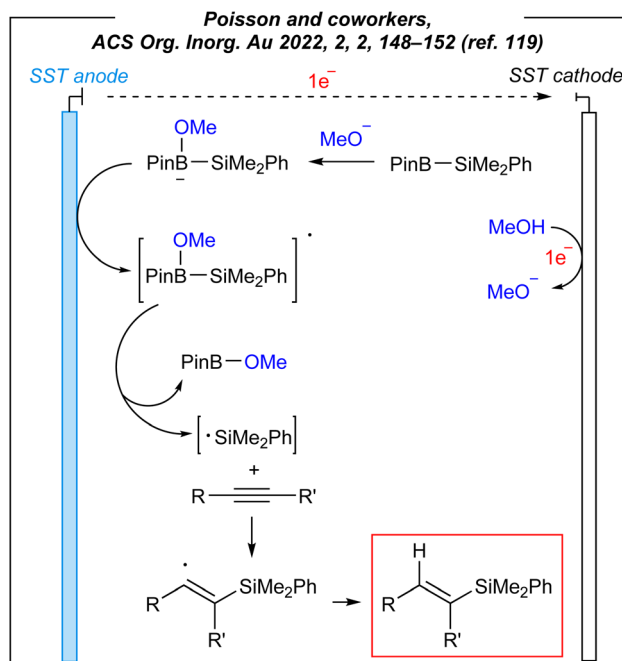
Fig. 15 Plausible mechanism for the electroinduced hydrosilylation.
