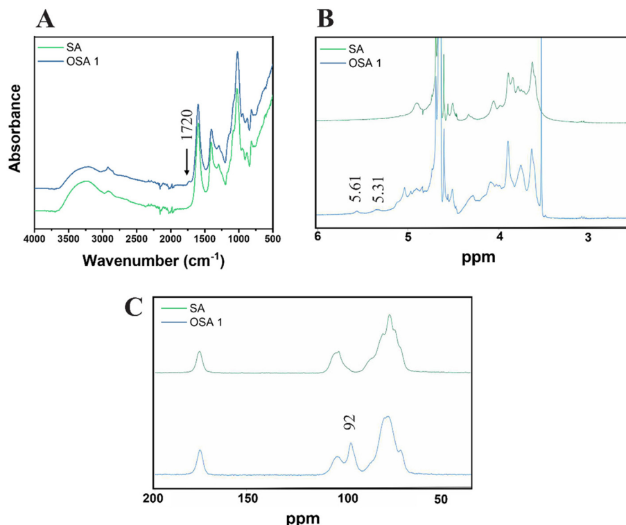
Fig. 2 ATR FT-IR (A), 1 H-NMR (B) and solid-state 13 C-NMR (C) of OSA 1.
