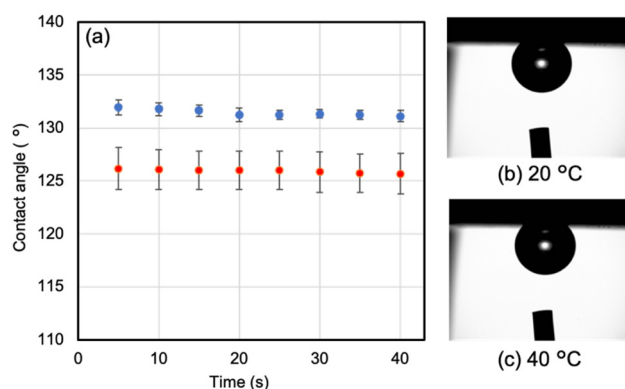
Fig. 3 (a) Contact angles of air-in-water (captive bubble) for the P(DEGMA- stat -TEGMA)/PMMA heteroarm star-shaped polymer-coated surface at 20 and 40 °C. Photographic images of the captive bubbles at (b) 20 °C and (c) 40 °C.
