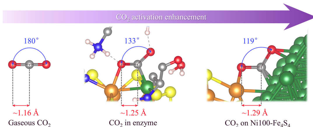
Fig. 2 Schematic diagram of the geometric structure of \text{CO}_2 in different adsorption states and \text{CO}_2 activation enhancement. (In atomic coloring, white is H, gray is C, blue is N, red is O, yellow is S, orange is Fe, and green is Ni).
