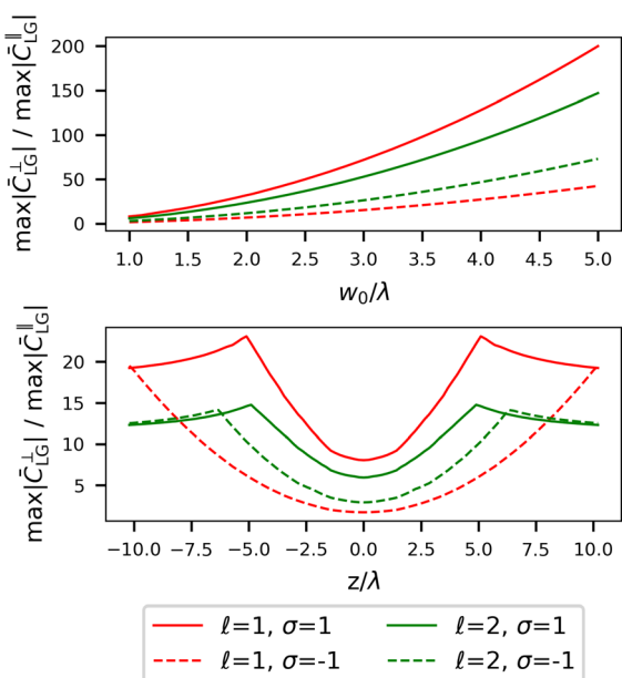
Fig. 7 Ratio of \max|\tilde{C}_{\text{LG}}^\perp|/\max|\tilde{C}_{\text{LG}}^\parallel| for p = 1 versus beam waist w_0 (top) and propagation distance from focal plane z = 0 (bottom). The increase in ratio as either the beam waist w_0 or distance from the focal plane increases highlights the rapid decrease in relative magnitude of the longitudinal fields with respect to the transverse fields, i.e. the fields essentially become completely transverse.
