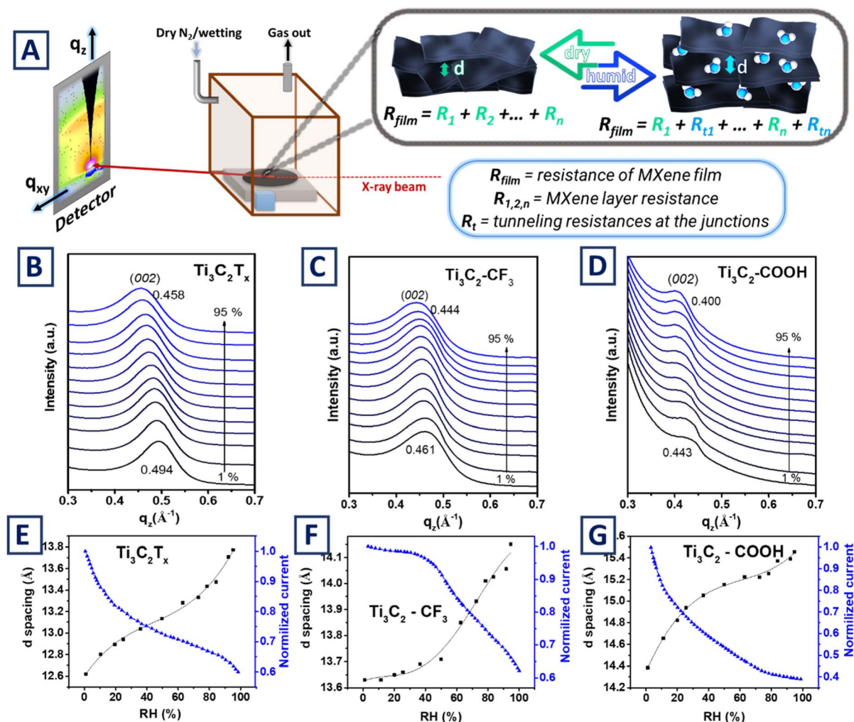
Fig. 4 (A) Schematic representation of GIWAXS in situ measurements of Ti 3 C 2 T x thin films response to humidity presence; (B)–(D) shifts of characteristic (002) XRD peak position of pristine and grafted Ti 3 C 2 T x films as a function of surrounding humidity level and flakes' surface terminations; (E)–(G) comparison of the changes of d -spacing of Ti 3 C 2 T x films and thin films conductivity changes, induced by the water molecules capture at different humidity levels.
