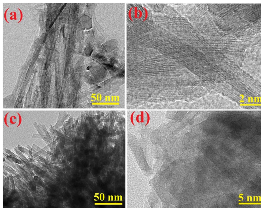
Fig. 6 TEM and HRTEM images of (a and b) pure \text{TiO}_2\text{NT} and (c and d) \text{TiO}_2\text{NT-AC} nanocomposites.
