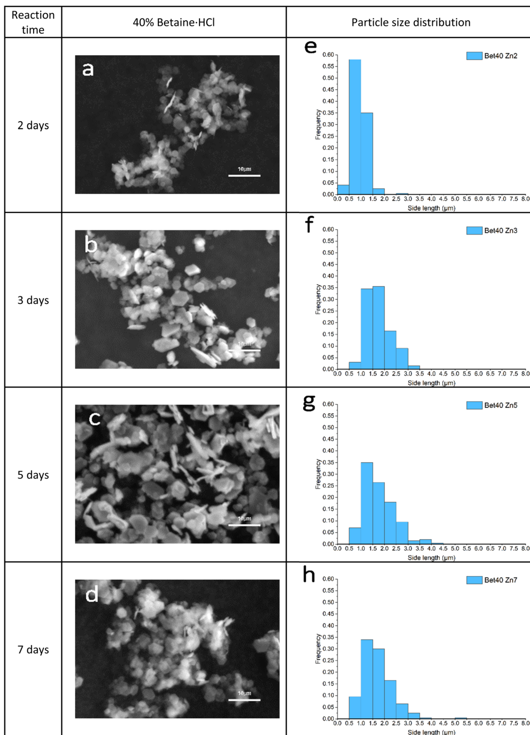
Fig. 9 (a–d) SEM images of simonkolleite crystal growth synthesised in 40% of betaine·HCl over time; (e–h) corresponded PSD maps statistical the side lengths of 200 hexagonal crystals.
