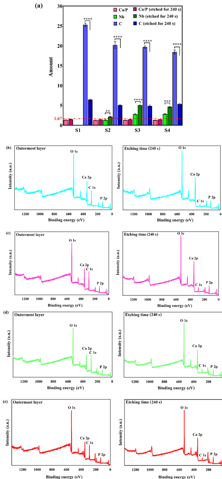
Fig. 6 (a) The XPS-derived data, including Ca/P ratio and atomic percent of Nb and C elements (** p = 0.0013 , *** p = 0.0001 , **** p < 0.0001 ); and XPS survey spectra of the outermost and subsurface layers: (b) S1, (c) S2, (d) S3, and (e) S4.
