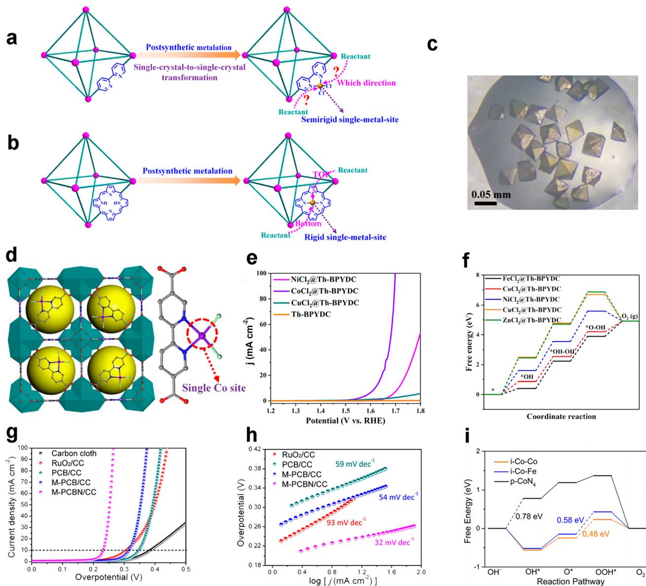
Fig. 7 MOF-based OER electrocatalysts. Routes of reactants accessible to the single-metal site in bipyrrolyl- (a) and porphyrin-MOFs (b); (c) optical microscopy image of \text{CoCl}_2\text{@Th-BPYDC} ; (d) crystal structure of \text{CoCl}_2\text{@Th-BPYDC} ; (e) LSV curves of \text{CoCl}_2\text{@Th-BPYDC} and other samples for OER tests in 0.1 M \text{HClO}_4 ; (f) calculated free energy diagram for the reaction transition state of the OER process for \text{CoCl}_2\text{@Th-BPYDC} and other samples. Reproduced with permission. 79 Copyright 2022, American Chemical Society; (g) LSV curves and (h) Tafel plot of M-PCBN/CC and other samples for OER tests in 1.0 M KOH; (i) calculated free energy per step diagrams of the OER for i-Co-Co, i-Co-Fe and p-CoN 4 at 1.23 V. Reproduced with permission. 80 Copyright 2020, American Chemical Society.
