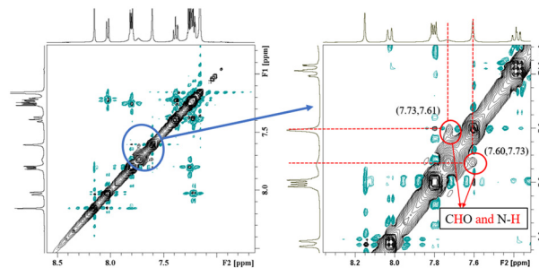
Fig. 5 The NOESY spectrum of 0.2 mg carbazole, 0.2 mg anthracene and 4.0 mg DMF in 400 \mu L C 6 D 6 at 8 °C.
