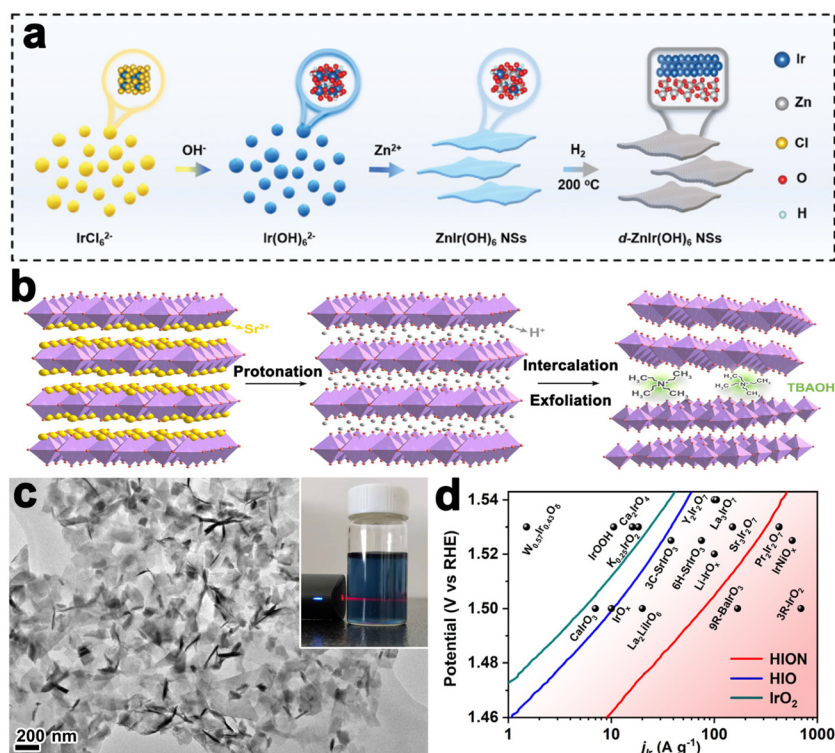
Fig. 5 (a) Schematic illustration of the synthesis of \text{ZnIr}(\text{OH})_6 NSs and \text{d-ZnIr}(\text{OH})_6 NSs (reproduced from ref. 92 with permission from the Royal Society of Chemistry, copyright 2022). 92 (b) Liquid-phase exfoliation of \text{Sr}_2\text{IrO}_4 . (c) TEM image of HION and the inset showing the photograph of HION colloidal suspension with typical Tyndall light scattering under laser irradiation. (d) Comparison of Ir mass activity of HION with previously reported OER catalysts in acid media (reproduced from ref. 93 with permission from the American Chemical Society, copyright 2022). 93
