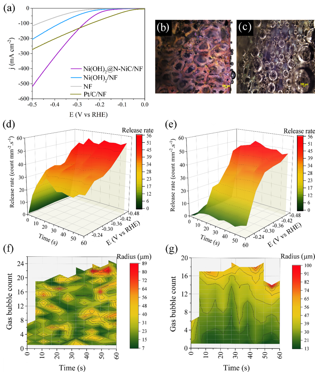
Fig. 2 (a) HER polarization curves. Optical images of gas bubbles over (b) \text{Ni}(\text{OH})_2@N\text{-NiC}/\text{NF} and (c) \text{Ni}(\text{OH})_2/\text{NF} at 0.245 V vs. RHE. Operando optical microscopy: 3D surface plots of (d) \text{Ni}(\text{OH})_2@N\text{-NiC}/\text{NF} and (e) \text{Ni}(\text{OH})_2/\text{NF} . Contour plots at 0.445 V vs. RHE for (f) \text{Ni}(\text{OH})_2@N\text{-NiC}/\text{NF} and (g) \text{Ni}(\text{OH})_2/\text{NF} .
