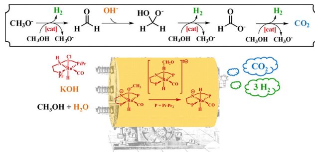
Fig. 8 The mechanism of \text{RuHCl}(\text{CO})(\text{HN}(\text{C}_2\text{H}_4\text{PiPr}_2)_2) catalyzed methanol dehydrogenation. 268 Reproduced with permission from ref. 268. Copyright (2016) American Chemical Society.
