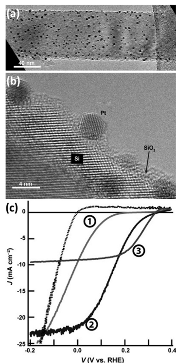
Fig. 10 (a) TEM and (b) HRTEM images of Pt nanoparticles modified Si nanowire, (c) PEC HER performance of naked Si nanowires (①), and Si nanowires modified with Pt nanoparticles prepared by ELD (②) and ALD (③). Reproduced with permission from ref. 86, Copyright © 2013 Wiley-VCH Verlag GmbH & Co. KGaA, Weinheim.
