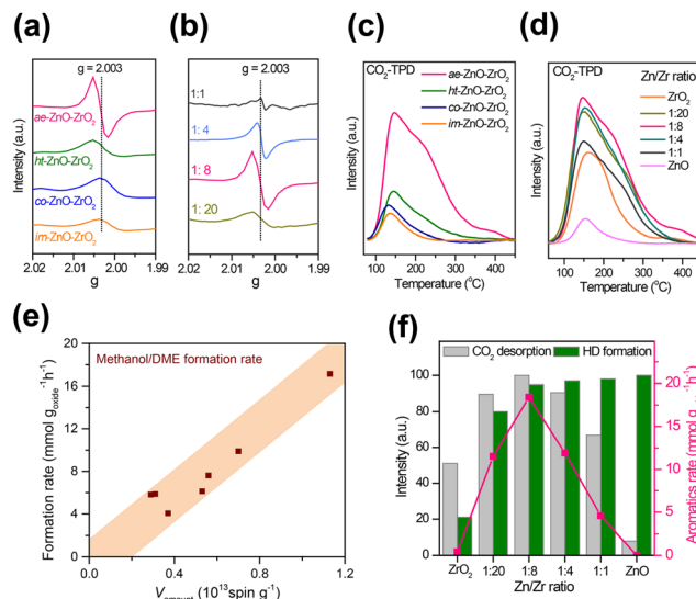
Fig. 10 EPR spectra of ZnO– \text{ZrO}_2 components with (a) different preparation methods and (b) Zn/Zr molar ratios, \text{CO}_2 -TPD curves of ZnO– \text{ZrO}_2 components with (c) different preparation methods, and (d) Zn/Zr molar ratios. (e) The dependence of the \text{CH}_3\text{OH}/\text{DME} formation rate on the total number of oxygen vacancies. (f) Normalized \text{CO}_2 desorption amounts and HD formation rates against the Zn/Zr molar ratio and the effect of the Zn/Zr molar ratio on the formation rate of aromatics. 98 Reproduced from ref. 98 with the permission from American Chemical Society, copyright 2019.
