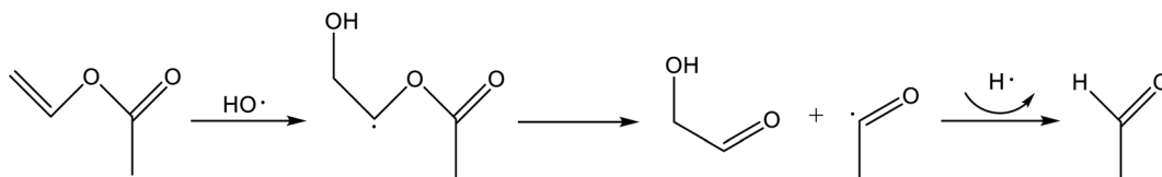
Fig. 2 Photocatalytic formation of acetaldehyde from vinyl acetate as proposed by Gandolfo et al. 69
