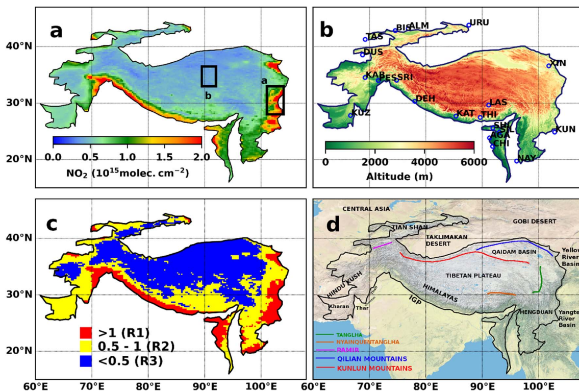
Fig. 1 (a) Mean (2005–2020) tropospheric NO 2 column (in 10^{15} molec. cm -2 ) in the TP. Box a represents the most polluted region and box b represents a pristine region in the TP. (b) Topography of the study region with selected cities marked in circles. (c) Mean (2005–2020) tropospheric NO 2 over the TP with three distinct ranges of NO 2 : regions with NO 2 less than 0.5 \times 10^{15} molec. cm -2 (blue colour), between 0.5 and 1 \times 10^{15} molec. cm -2 (yellow colour), and greater than 1 \times 10^{15} molec. cm -2 (red colour). (d) The geographic map of the TP and adjacent regions (no country borders marked).
