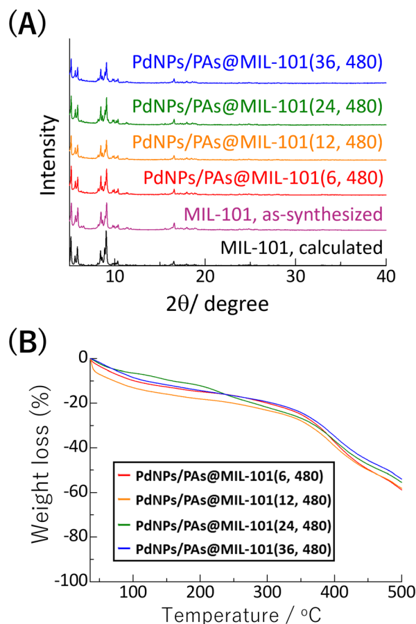
Fig. 2 (A) XRD data and (B) TG profiles of \text{PdNPs}/\text{PAs}@\text{MIL-101}(x, 480) ( x = 6, 12, 24, 36 ).
