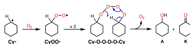
Scheme 2 Russell rearrangement.
