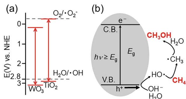
Fig. 9 Typical photocatalytic partial oxidation of methane to methanol mechanism catalyzed by metal oxide. (a) Redox potentials of WO 3 and TiO 2 . (b) Mechanism of the conversion of CH 4 to CH 3 OH by photocatalytic reaction. Adapted with permission from ref. 84 under the terms of the CC BY 3.0 license.
