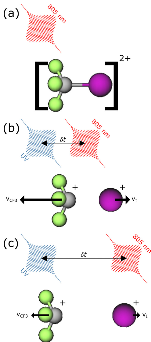
Fig. 12 Illustration of the sources of important signatures evident in UV pump -805\text{ nm} SFI probe experiments at different time delays, \delta t , using \text{CF}_3\text{I} as the exemplar and assuming removal of two electrons and a symmetric charge separation. (a) \text{CF}_3\text{I}^{2+} formation by 805\text{ nm} SFI alone, or with the UV and 805\text{ nm} pulses coincident in time ( i.e. \delta t = 0 ). The subsequent CE of these dications results in the \text{CF}_3^+ and \text{I}^+ products identified with the label ISFI in the respective 2-D maps. (b and c) \text{CF}_3^+ and \text{I}^+ fragments formed by 805\text{ nm} SFI (at progressively later delays \delta t ) of neutral \text{CF}_3 and \text{I} products formed by UV excitation at t = 0 . The neutral photoproducts are formed with characteristic, thermochemically determined, recoil velocities (equal to that of the feature(s) labelled DISS in the 2-D maps). Subsequent SFI of these neutral fragments introduces an additional Coulombic repulsive contribution to the measured \text{CF}_3^+ and \text{I}^+ velocities, the magnitude of which decreases with increasing \delta t ( i.e. increasing inter-ion separation) as illustrated by the velocity vectors in (b and c). This process is responsible for the characteristic DCE signals, the velocities of which converge to that of the DISS component at long \delta t .
