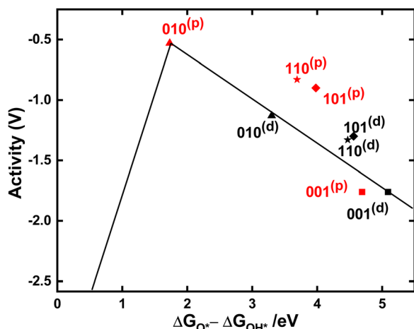
Fig. 5 Volcano plot ( -\eta vs. \Delta G_{O\bullet} - \Delta G_{OH\bullet} ) for the oxygen evolution reaction on low-indexed TiO_2 surfaces explored in this study. The data points are grouped with black color for dangling O^{(d)} and red color for peroxo O^{(p)} .
