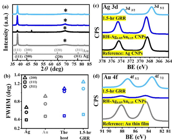
Fig. 4 Characterization of the host RH-Ag 0.85 Au 0.15 CNPs and the RH-Ag: Au m-CNPs (produced by the 1.5 h-GRR of the host at T_{AL} = 20 nm) with (a) XRD and (c) and (d) XPS. (b) Plot of the full width of half maximum (FWHM) of the (111), (200) and (311) facets measured in (a). (a) The peaks marked with asterisks are assigned to the silicon wafers on which the CNPs are deposited. XPS: (c) Ag 3d; (d) Au 4f. Black and grey symbols: RH-Ag CNPs and Au thin films, respectively (as references); blue symbols: the host; cyan symbols: RH-Ag: Au m-CNPs.
