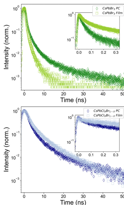
Fig. 3 Time-resolved photoluminescence (TRPL) dynamics of neat PNC films and PC \subset PNCs. PL decay traces of: (A) C_{s}PbBr_{3} NCs ( \lambda_{ex} = 390 nm). (B) C_{s}PbCl_{1.5}Br_{1.5} NCs ( \lambda_{ex} = 350 nm).
