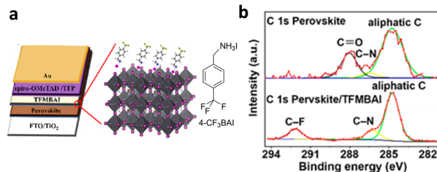
Fig. 28 (a) The passivation of the triple cation perovskite with 4-CF 3 BAI. (b) XPS spectrum showing disappearance of the C=O peak upon passivation. 130 Reproduced with permission from ref. 130. Copyright 2021, American Chemical Society.
