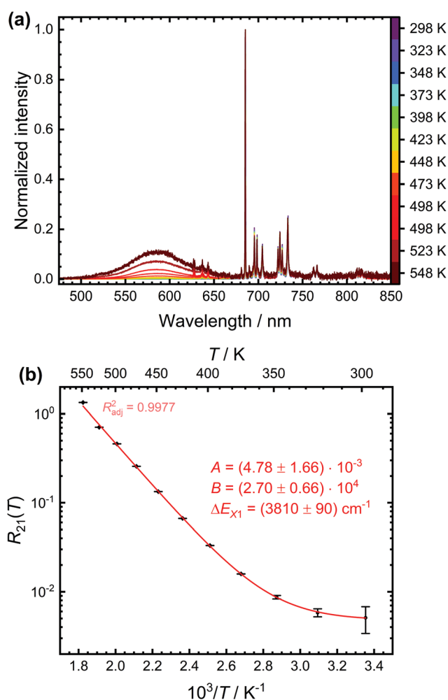
Fig. 4 (a) Temperature-dependent emission spectra of \text{SrB}_4\text{O}_7:0.5\% \text{Sm}^{2+} ( \lambda_{\text{ex}} = 423 nm) normalized to the intensity of the most intense ^5\text{D}_0 \rightarrow ^7\text{F}_0 transition. The peaks on the top of the broad 4f^55d^1 \rightarrow 4f^6 -based emission band stem from the ^5\text{D}_1 \rightarrow ^7\text{F}_J ( J = 0, 1, 2 )-related emission. (b) Data (black points) and least-squares fit (red line) according to eqn (4) of the temperature-dependent luminescence intensity ratio between the 4f^55d^1 \rightarrow 4f^6 - and ^5\text{D}_0 \rightarrow ^7\text{F}_J -based emission. The fitting parameters and the adjusted (squared) correlation coefficient indicating the quality of the fit is given as well.
