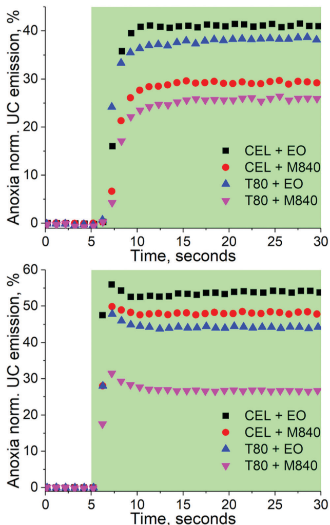
Fig. 3 Deoxygenation curves of the nanocarriers under 260 (top) and 1000 \text{mW cm}^{-2} excitation. The green sections indicate the time under excitation, i.e. the excitation was started after the first 5 seconds. The data is normalized by the emission intensity obtained at anoxic conditions. The emission spectra recorded at the 30 s mark are shown in Fig. S4 and S5 (ESI † ).
