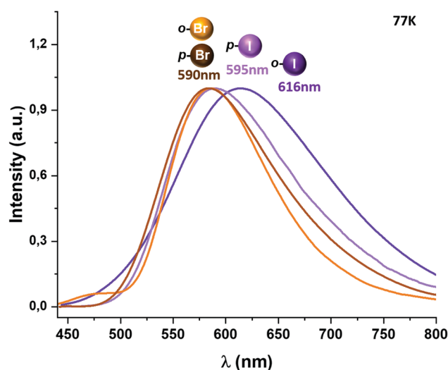
Fig. 5 Excitation and emission spectra of complexes [Au(o-C 6 BrF 4 )(dppBz)] (2) (orange), [Au(p-C 6 BrF 4 )(dppBz)] (3) (brown), [Au(o-C 6 F 4 I)(dppBz)] (4) (purple) and [Au(p-C 6 F 4 I)(dppBz)] (5) (light purple) in the solid state measured at 77 K.
