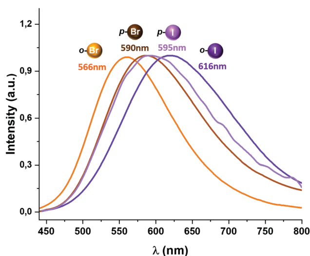
Fig. 4 The excitation and emission spectra in the solid state of the complexes [Au(o-C 6 BrF 4 )(dppBz)] (2) (orange), [Au(p-C 6 BrF 4 )(dppBz)] (3) (brown), [Au(o-C 6 F 4 I)(dppBz)] (4) (purple) and [Au(p-C 6 F 4 I)(dppBz)] (5) (light purple) measured at room temperature.
