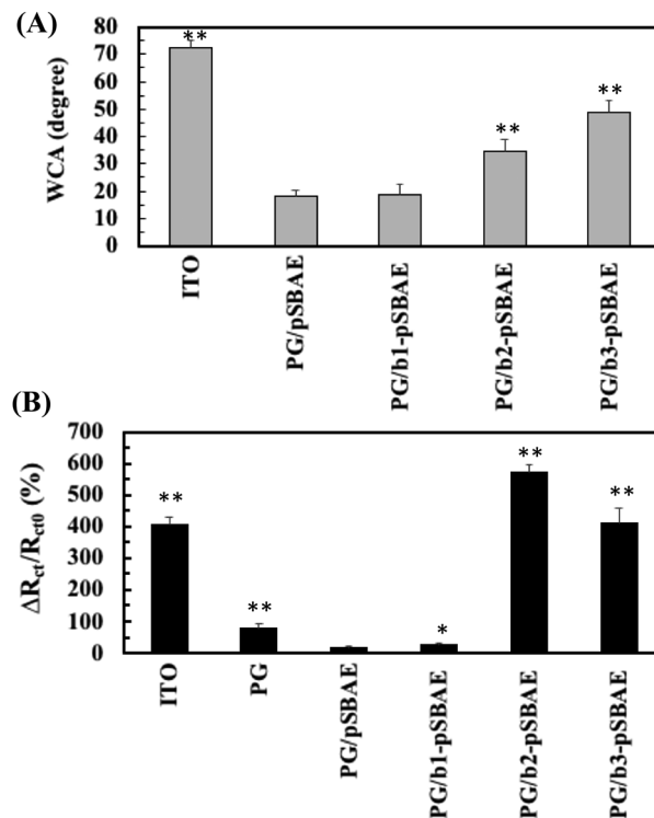
Fig. 5 (A) Static water contact angles of PG/b-pSBAE electro-deposited ITO for 4 CV cycles. PG/b-pSBAE = 8/30 \text{mg mL}^{-1} . (B) ITO and PG/pSBAE modified ITO was incubated in 0.1 \text{mg mL}^{-1} of avidin for 2 hours and the changes in charge transfer resistance were determined. * and ** represent p < 0.05 and < 0.001 , compared to PG/pSBAE, respectively. Value = mean \pm standard deviation, n = 3 .
