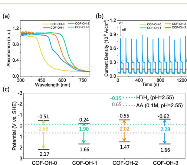
Fig. 3 UV-vis diffuse reflectance spectra of COF-OH-0-3 (a); photocurrent-time curves under \lambda \geq 420 nm light irradiation of COF-OH-0-3 (b); band position and bandgap of COFs vs. the standard hydrogen electrode (SHE) along with the potential of H + /H 2 and one-hole (HA • /H 2 A) oxidation of L-ascorbic acid under current conditions (c).
