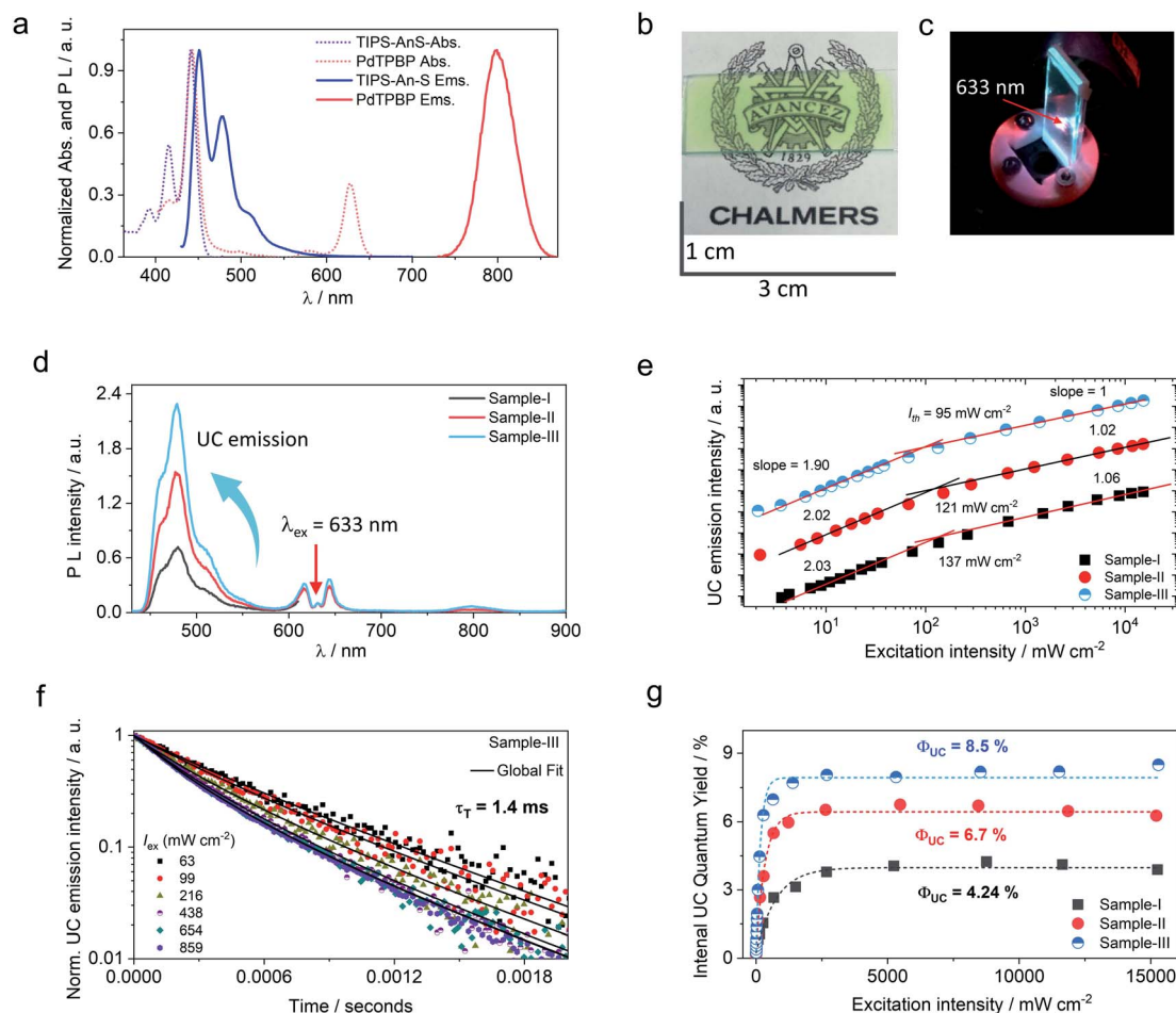
Fig. 3 Optical characterization of G-TXr-TIPS-AnS-PdTPBP film. (a) Absorption (dotted lines) and PL (solid lines) spectra of the G-TXr-TIPS-AnS (blue line, \lambda_{ex} = 415 nm, TIPS-AnS = 200 \mu mol kg -1 ) and G-TXr-PdTPBP (red line, \lambda_{ex} = 633 nm, 27 \mu mol kg -1 ) films in the air. (b) Photograph of G-TXr-TIPS-AnS-PdTPBP film under white light, and (c) under 633 nm laser excitation in the air (excitation intensity = 1.3 W cm -2 , no short pass filter used). (d) Comparative PL spectra of G-TXr-PdTPBP-TIPS-AnS films at different concentrations of TIPS-AnS (1, 2.5 and 5 mmol kg -1 ) upon 633 nm laser excitation (excitation intensity = 33.8 mW cm -2 ). (e) Comparative log-log plot of excitation intensity dependence of UC emission intensity of G-TXr-TIPS-AnS-PdTPBP films at different concentrations of TIPS-AnS. (f) Time traces of normalized upconversion emission intensity of G-TXr-TIPS-AnS-PdTPBP sample-III for various excitation intensities in the air ( \lambda_{ex} = 633 nm laser, \lambda_{em} = 478 nm). (g) Comparative internal UC quantum yield of G-TXr-TIPS-AnS-PdTPBP films in the air.
