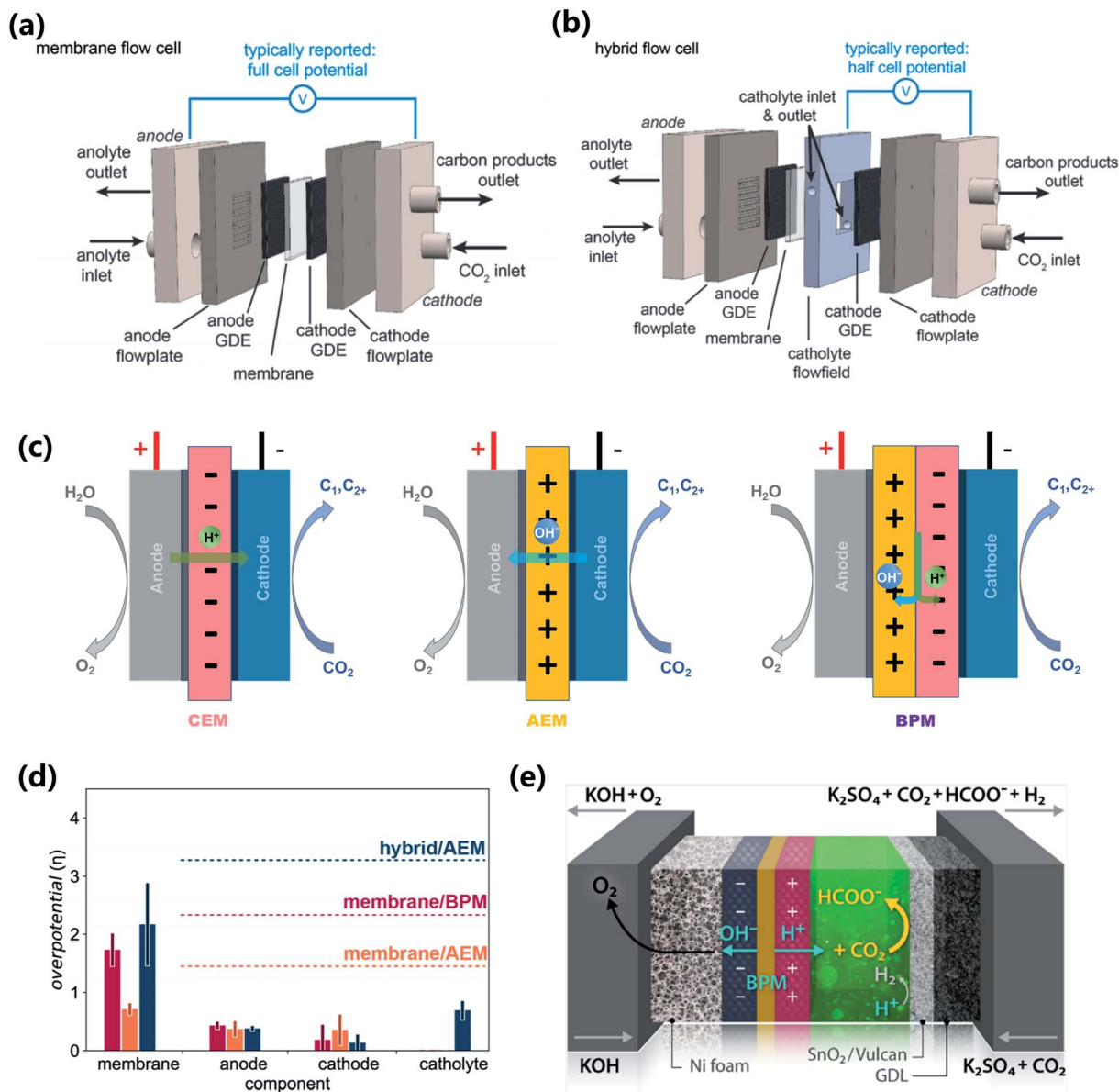
Fig. 9 (a and b) Schematic illustrations of the zero-gap membrane flow cell and hybrid flow cell. Adapted with permission. 154 Copyright 2019, American Chemical Society. (c) Schematic illustrations of electrolytic flow cells with an AEM, CEM and BPM. (d) Overpotentials at 200 \text{ mA cm}^{-2} for each of the functional components in membrane/BPM (red), membrane/AEM (orange), and hybrid/AEM (navy). Adapted with permission. 154 Copyright 2019, American Chemical Society. (e) Schematic illustration of a novel cell with a thin layer of catholyte buffer. Adapted with permission. 159 Copyright 2020, American Chemical Society.
