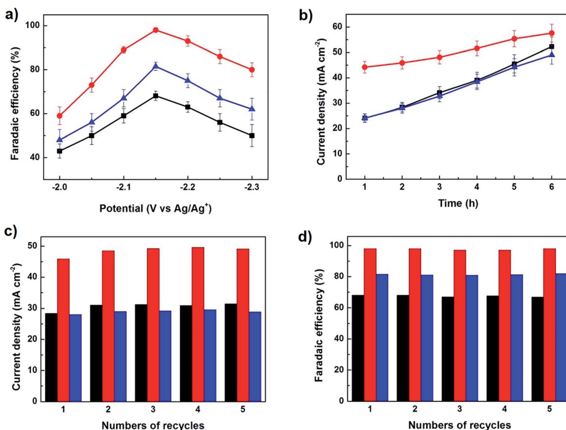
Fig. 6 Electrochemical CO 2 RR performance of MFM-300(In) prepared via different synthesis methods by Kang et al. (ref. 99): electrochemical synthesis over an In foil (red), electrochemical synthesis followed by deposition over carbon paper (blue) and solvothermal synthesis and drop casting over carbon paper (black). (a) Shows faradaic efficiency towards the formation of HCOOH, (b) plots the current density in a constant potential electrolysis, and (c) and (d) convey the change in current density and faradaic efficiency in five cycles of a 2 h constant potential electrolysis at -2.15 V (vs. Ag/Ag + ) (reproduced with permission from ref. 99. Copyright American Chemical Society 2020, further permissions related to the material excerpted should be directed to the ACS).
