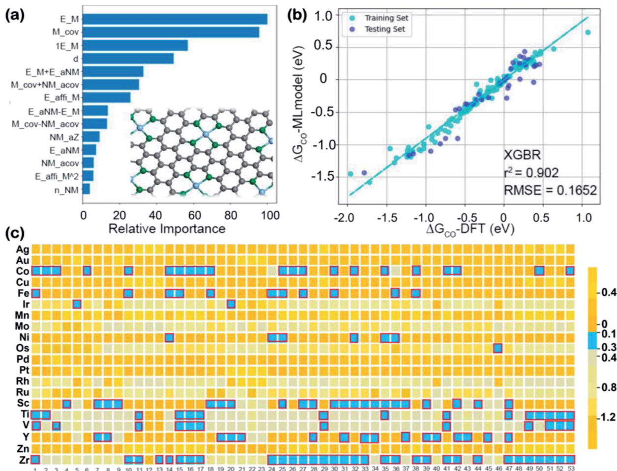
Fig. 8 Machine Learning for the CO 2 RR. (a) Feature importance analysis for \Delta G_{CO^*} prediction using ML. Pauling electronegativity (E_M), covalent radius (M_cov), and first ionization energy of transition metal atoms as SACs (1E_M) are the most important parameters. The inset shows the structures of SACs used for the CO 2 RR. Green, gray, and blue spheres indicate nonmetal, carbon, and transition metal atoms, respectively. (b) Comparison of ML- and DFT-predicted \Delta G_{CO^*} . (c) High-throughput screening of \Delta G_{CO^*} using XGBR models. Reproduced with permission from ref. 160, copyright 2020, American Chemical Society. These figures indicate that ML can accurately predict \Delta G_{CO^*} for the better design of SACs.
