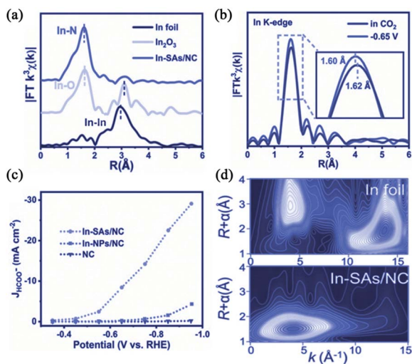
Fig. 8 (a) In K-edge spectra of In-SAs/NC, In 2 O 3 and In foil; (b) in situ spectra of In-SAs/NC; (c) the current density of HCOO - in CO 2 RR; (d) WT-EXAFS spectra. Reprinted with permission from ref. 114. Copyright 2020, WILEY-VCH GmbH.
