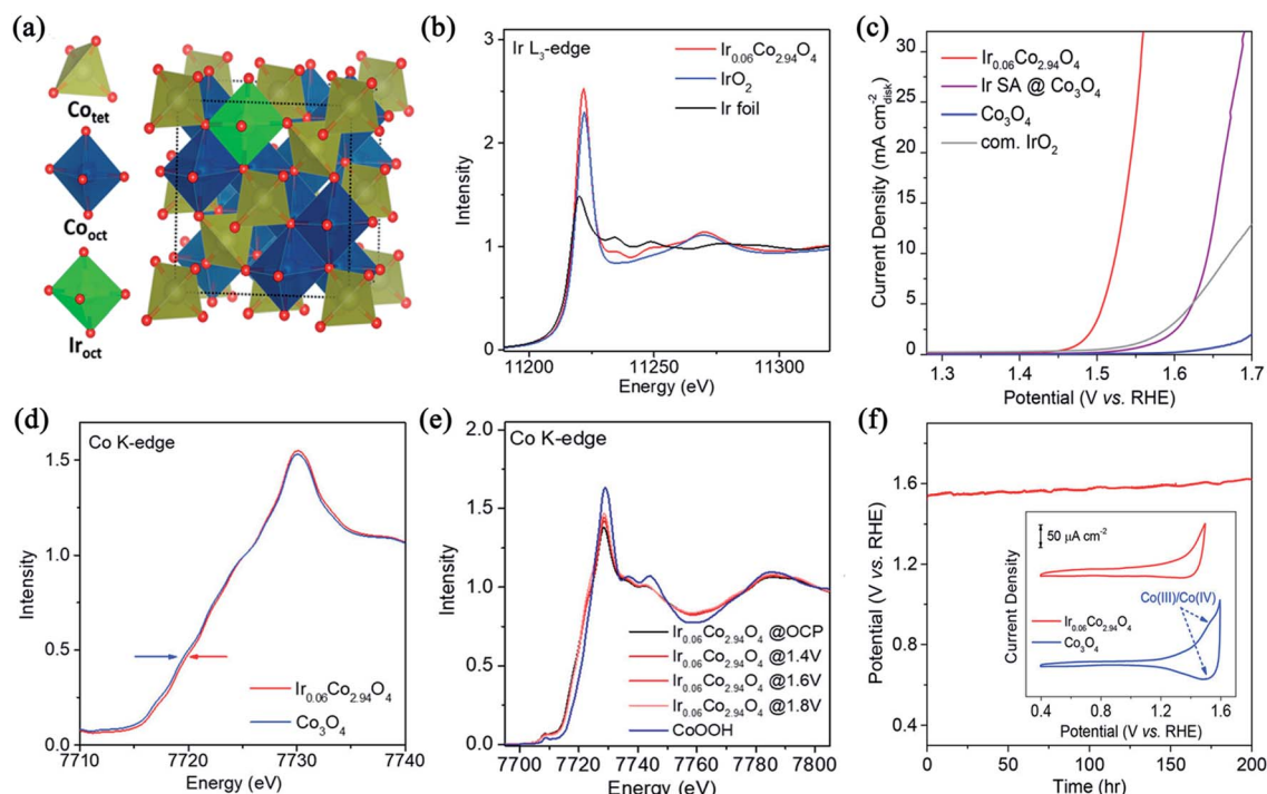
Fig. 4 (a) Structural model of Ir-substituted cobalt spinel oxide in a polyhedral representation; (b) Ir L 3 -edge spectra of Ir 0.06 Co 2.94 O 4 , IrO 2 and Ir foil; (c) polarization curves in O 2 -saturated 0.1 M HClO 4 ; (d) Co K-edge spectra of Ir 0.06 Co 2.94 O 4 and Co 3 O 4 support; (e) in situ Co K-edge spectra under several potentials; (f) chronopotentiometric curve of Ir 0.06 Co 2.94 O 4 at 10 mA cm -2 , the insert is cyclic voltammetry (CV) tests. Reprinted with permission from ref. 92. Copyright 2021, American Chemical Society.
