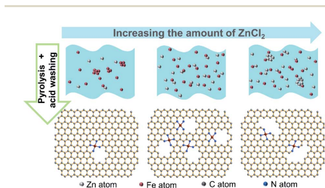
Fig. 3 Diagrammatical presentation of the influence of initial Zn/Fe molar ratio on the obtained catalysts.
