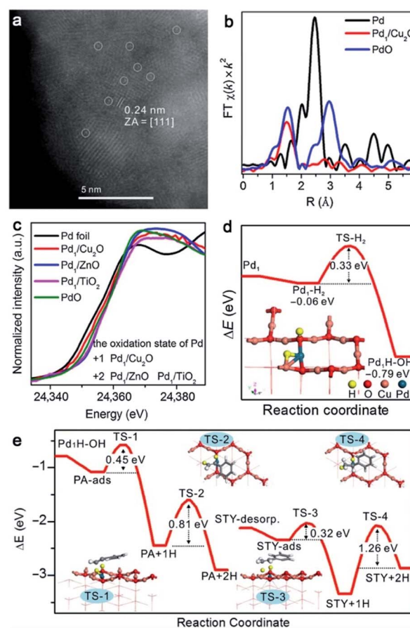
Fig. 5 (a) HAADF-STEM image of Pd 1 /Cu 2 O. (b) EXAFS spectra at the Pd K-edge of Pd 1 /Cu 2 O, Pd foil, and PdO. (c) XANES spectra of Pd catalysts on various supports, Pd foil, and PdO. (d) Energies and model of Pd 1 /Cu 2 O in the heterolytic activation of H 2 . (e) Energies of intermediates and transition states for hydrogenation of phenylacetylene on Pd 1 /Cu 2 O. Reproduced from ref. 71, published in CCS Chemistry 2019; Cu 2 O-supported atomically dispersed Pd catalysts for semihydrogenation of terminal alkynes: critical role of oxide supports is available online (DOI: 10.31635/ccschem.019.20190008).
