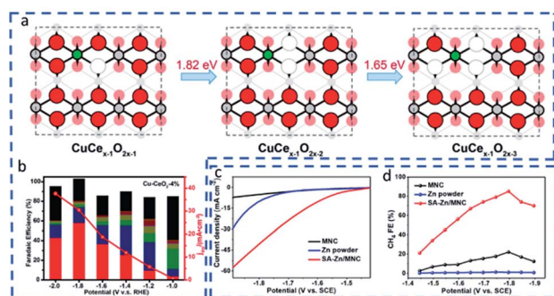
Fig. 7 (a) Stable structure model for Cu-SA/CeO 2 catalysts from DFT calculations. (b) FE CO of the Cu-SA/CeO 2 catalysts at different reduction potentials (red columns represent CH 4 and brown columns represent H 2 ). Reprinted with permission from ref. 98 Copyright 2018, the American Chemical Society. (c) Linear sweep voltammetry curves of Zn-N 4 -C in ECR. (d) FE CH 4 of Zn-N 4 -C SACs at different reduction potentials. Reprinted with permission from ref. 99 Copyright 2020, the American Chemical Society.
