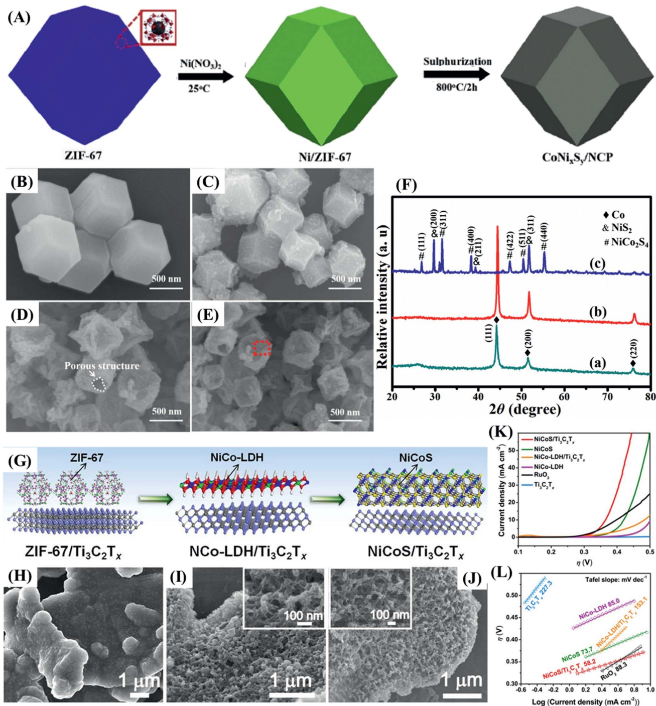
Fig. 22 (A) Scheme showing the fabrication of the CoNi x S y /NCP composite. SEM images of (B) ZIF-67, (C) Co/NC, (D) CoNi x /NCP, and (E) CoNi x S y /NCP. (F) XRD patterns of (a) Co/NC, (b) CoNi x S y /NCP, and (c) CoNi x S y /NCP. Adapted with permission from ref. 103. Copyright© 2019 Hydrogen Energy Publications LLC. Published by Elsevier Ltd. All rights reserved. (G) Scheme depicting the preparation of NiCoS/Ti 3 C 2 T x . SEM images of (H) ZIF-67/Ti 3 C 2 T x , (I) NiCo-LDH/Ti 3 C 2 T x , and (J) NiCoS/Ti 3 C 2 T x . Inset: the high-magnification SEM images of the samples. (K) LSV curves and (L) Tafel plots of NiCoS/Ti 3 C 2 T x , NiCoS, NiCo-LDH/Ti 3 C 2 T x , NiCo-LDH, and RuO 2 . Reproduced with permission from ref. 104. Copyright© 2018, American Chemical Society.
